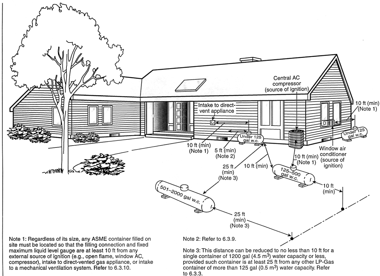
FIGURE I.1(b) Aboveground ASME Containers. (This figure for illustrative purposes only; code shall govern.)
